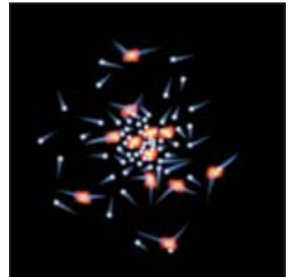
3 Eventually the gas settles down into hydrostatic equilibrium, with the density highest near the center of gravity.
