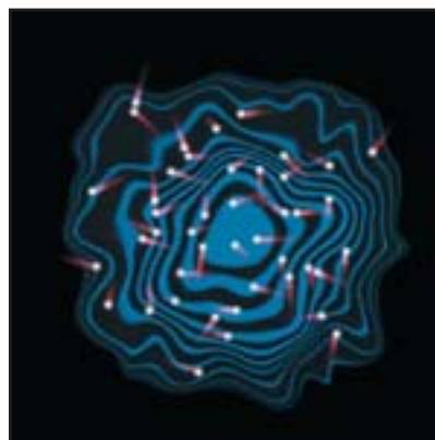
2 As the particles move around, the gravitational field changes, which causes particles to gain or lose energy.
