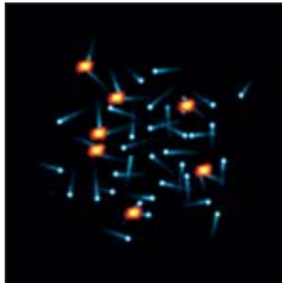
2 The gas particles bang into one another, redistributing energy and generating a pressure that resists gravity.
