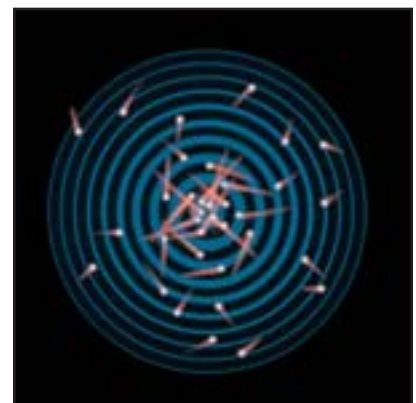
3 Gradually the system settles down into virial equilibrium, in which the gravitational field no longer fluctuates.
