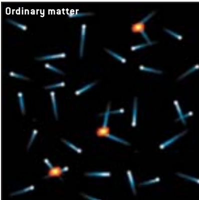
1 The ordinary matter—predominantly hydrogen gas—starts off moving every which way. Its density varies randomly.
