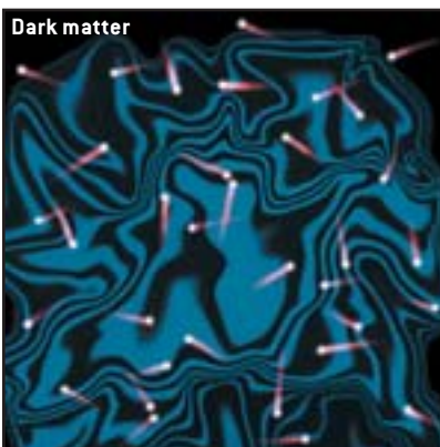
1 Initially the dark matter has the same arrangement as ordinary matter. The difference is that particles do not collide.
