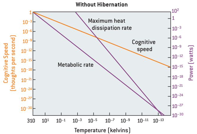
ETERNAL LIFE ON FINITE ENERGY? If a new form of life could lower its body temperature below the human value of 310 kelvins (98.6 degrees Fahrenheit), it would consume less power, albeit at the cost of thinking more sluggishly (left graph). Because metabolism would decline faster than cognition, the life-form could arrange to have an infinite number of thoughts on limited resources. One caveat is that its ability to dissipate waste heat would also decline, preventing it from cooling below about
