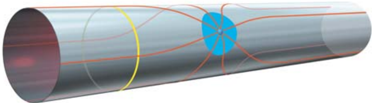
SMALL EXTRA DIMENSION wrapped in a circle ( circumference of tube ) modifies how gravity ( red lines ) spreads in space. At distances smaller than the circle radius ( blue patch ), the lines of force spread apart
